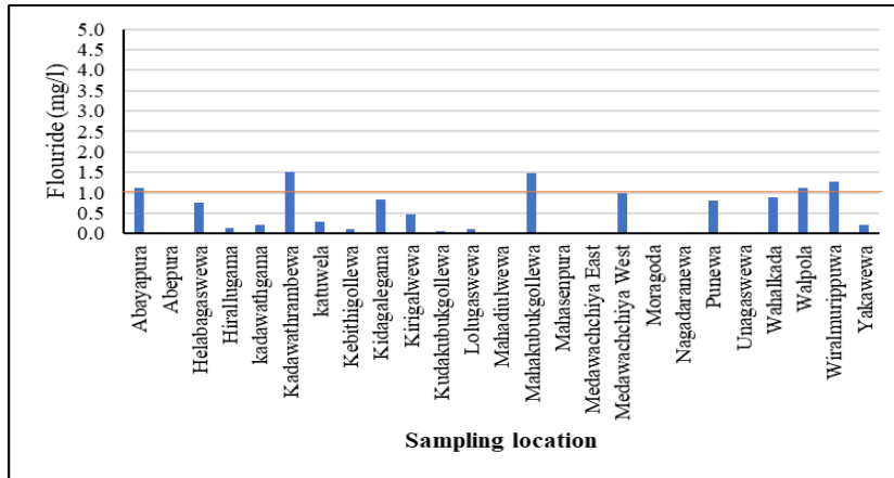
Fig. 9. Variation of Flouride in groundwater in the study area
