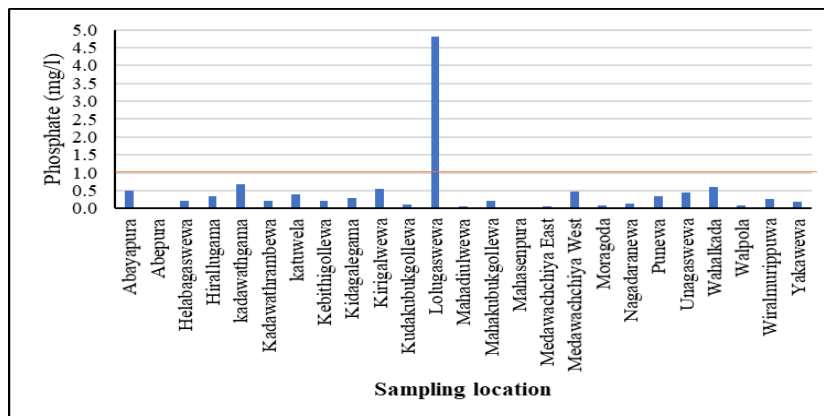
Fig. 11. Variation of Total Phosphate in groundwater in the study area
