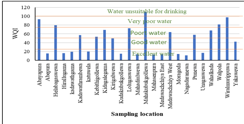
Fig. 12. Variation of WQI in groundwater in the study area
