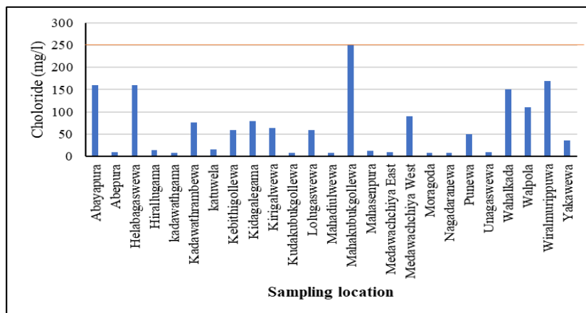
Fig. 6. Variation of Chloride in groundwater in the study area
