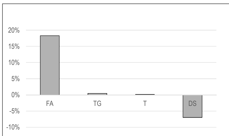
Figure 3.1.2. Mean Effects of the Different Factors on Iron Leaching
