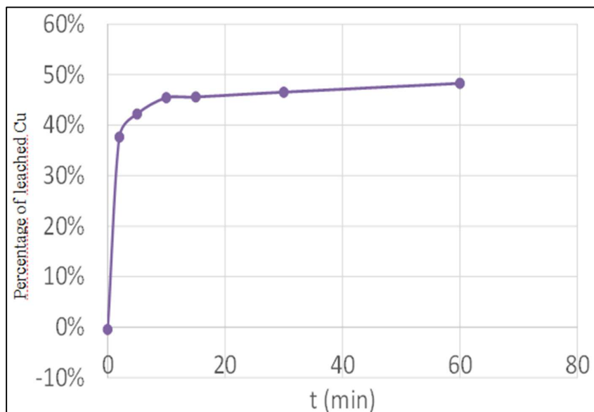
Figure 3.2.1. Kinetic Data of Cu Leaching at T = 60°C (AF = 0.40 mol·dm -3 , SD = 0.125, S = 500 rpm)
