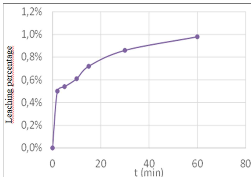
Figure III.3.2.2. Kinetic data for Fe leaching at T = 60^{\circ}\text{C} ( \text{FA} = 0.40 \text{ mol}\cdot\text{dm}^{-3} , \text{DS} = 0.125 , V = 500 \text{ rpm} )
