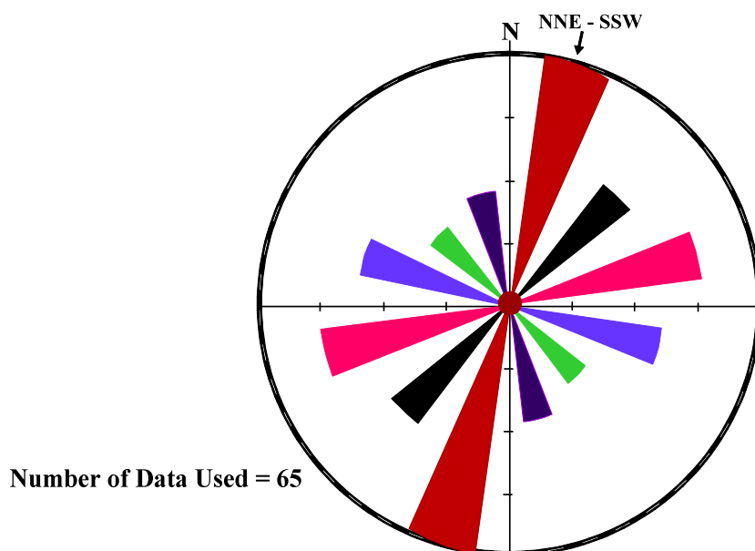
Figure 5: Rose Diagram Plot for Joints and Veins Pattern in Porphyritic Granite
