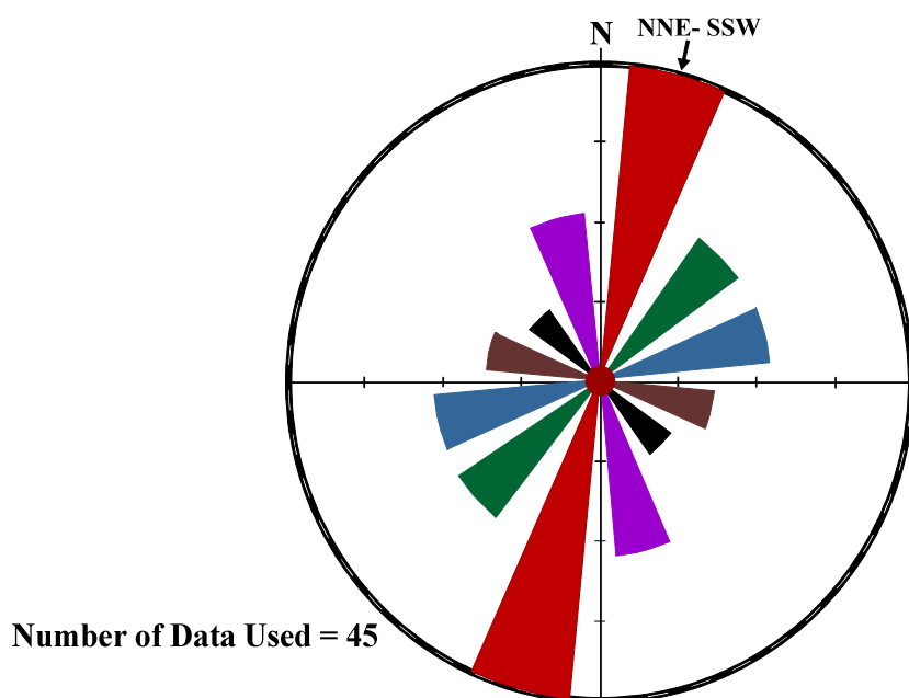
Figure 6: Rose Diagram Plot for Foliation Pattern in Granite-Gneiss
