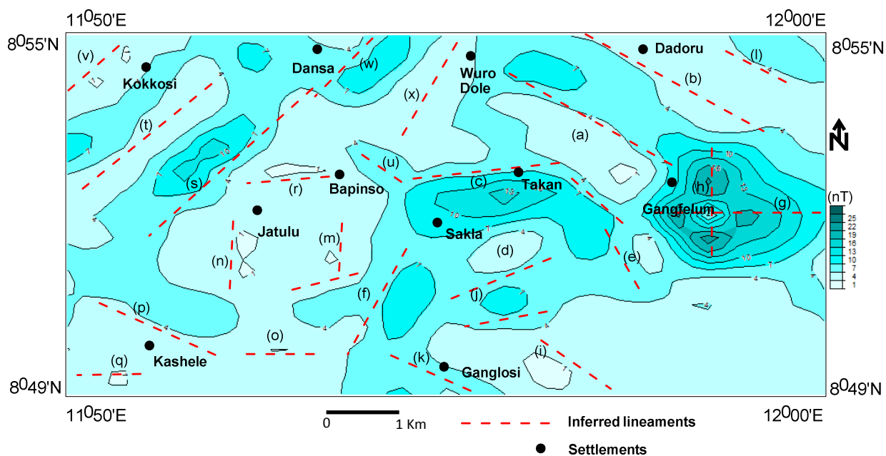
Figure 9. Horizontal Derivatives map of the study area with inferred lineaments (Cont. int. 3nT)
