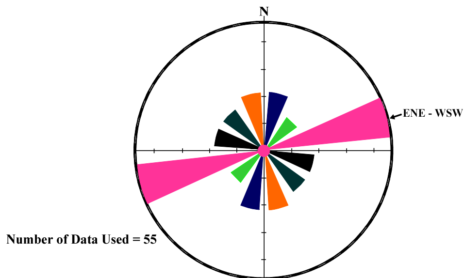
Plate II: Shows Foliations in Biotite Hornblende Gneiss in the Study Area
