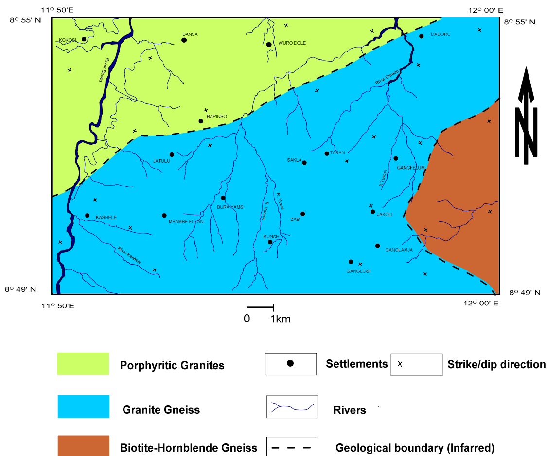
Figure 4: Geology of the study area (part of Adamawa Massifs) Northeastern Nigeria (from the present Study).
