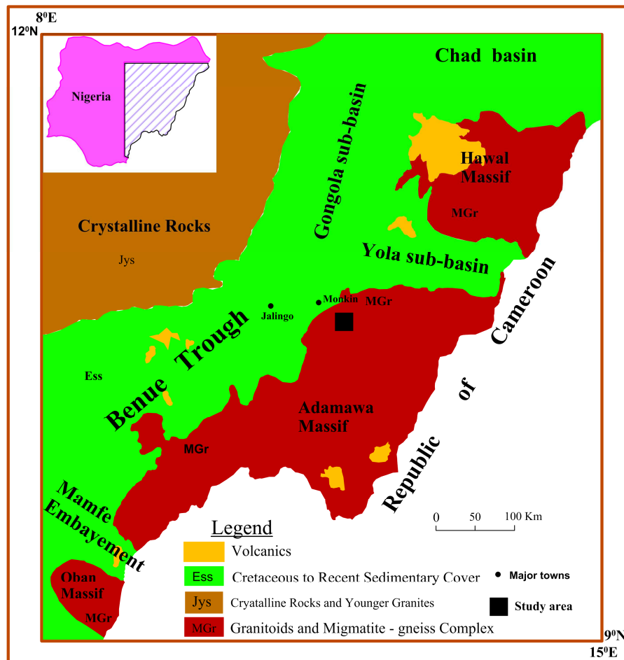
Figure 2: Regional Geological Setting of Adamawa Massif (Modified from [7]).
