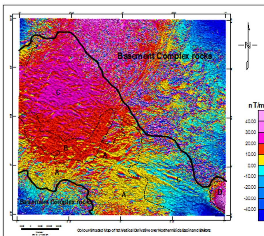
Fig. 5: Colour Shaded Map of 1 st Vertical Derivative over Northern Bida Basin and Environs
