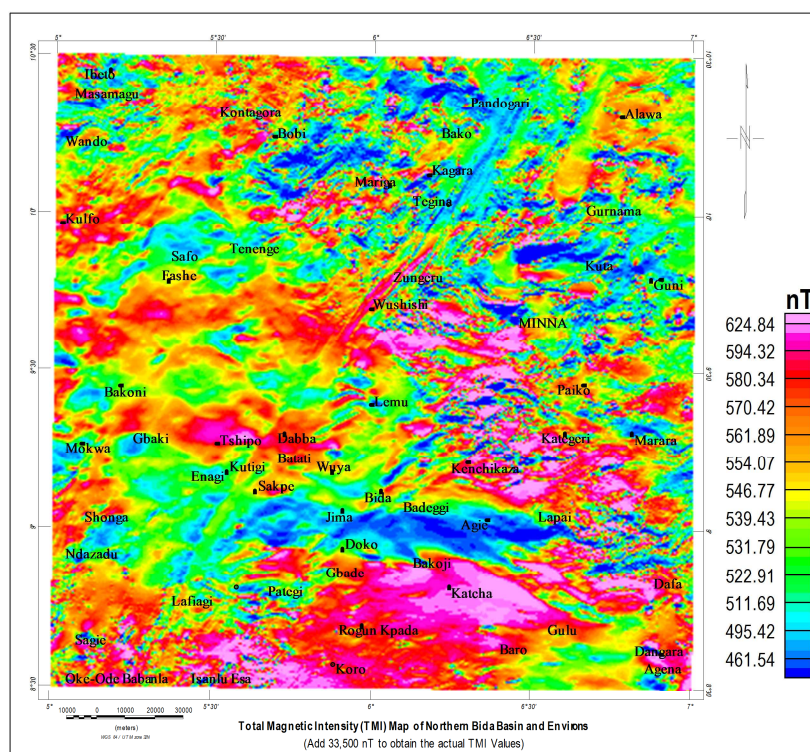
Fig. 2: Total Magnetic Intensity (TMI) Map of Northern Bida Basin and Environs
