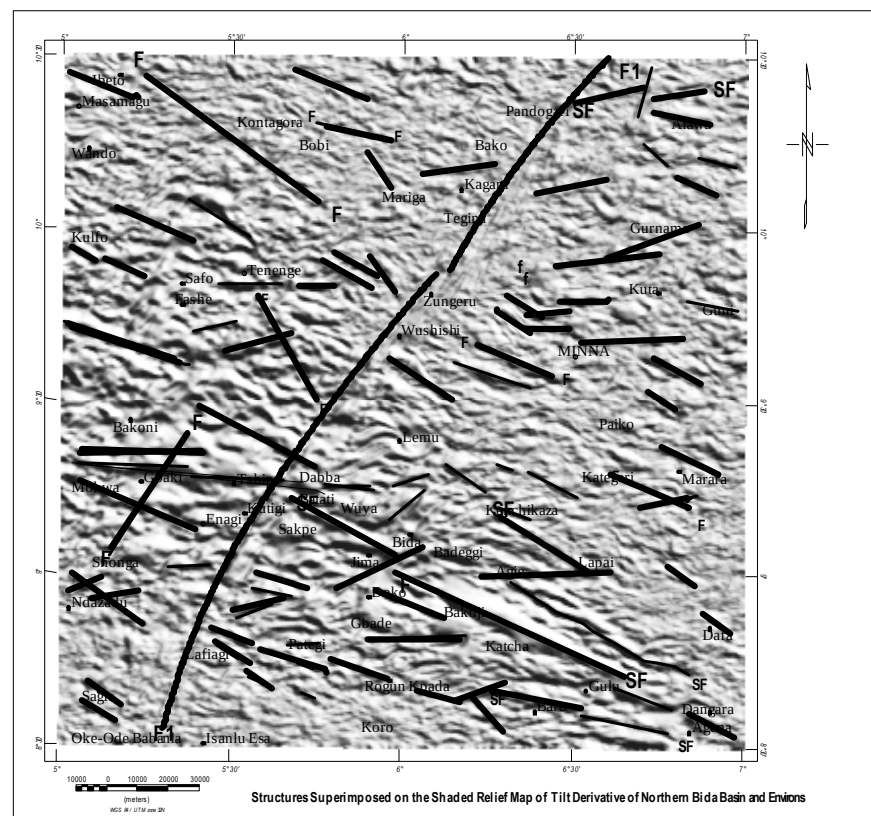
Fig. 8: Structures Superimposed on the Shaded Relief Map of Tilt Derivative
