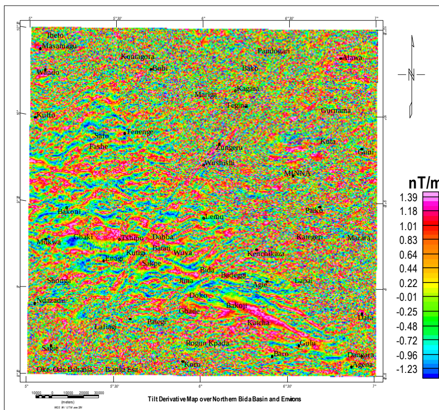
Fig. 6: Tilt Derivative Map draped on the Study Area
