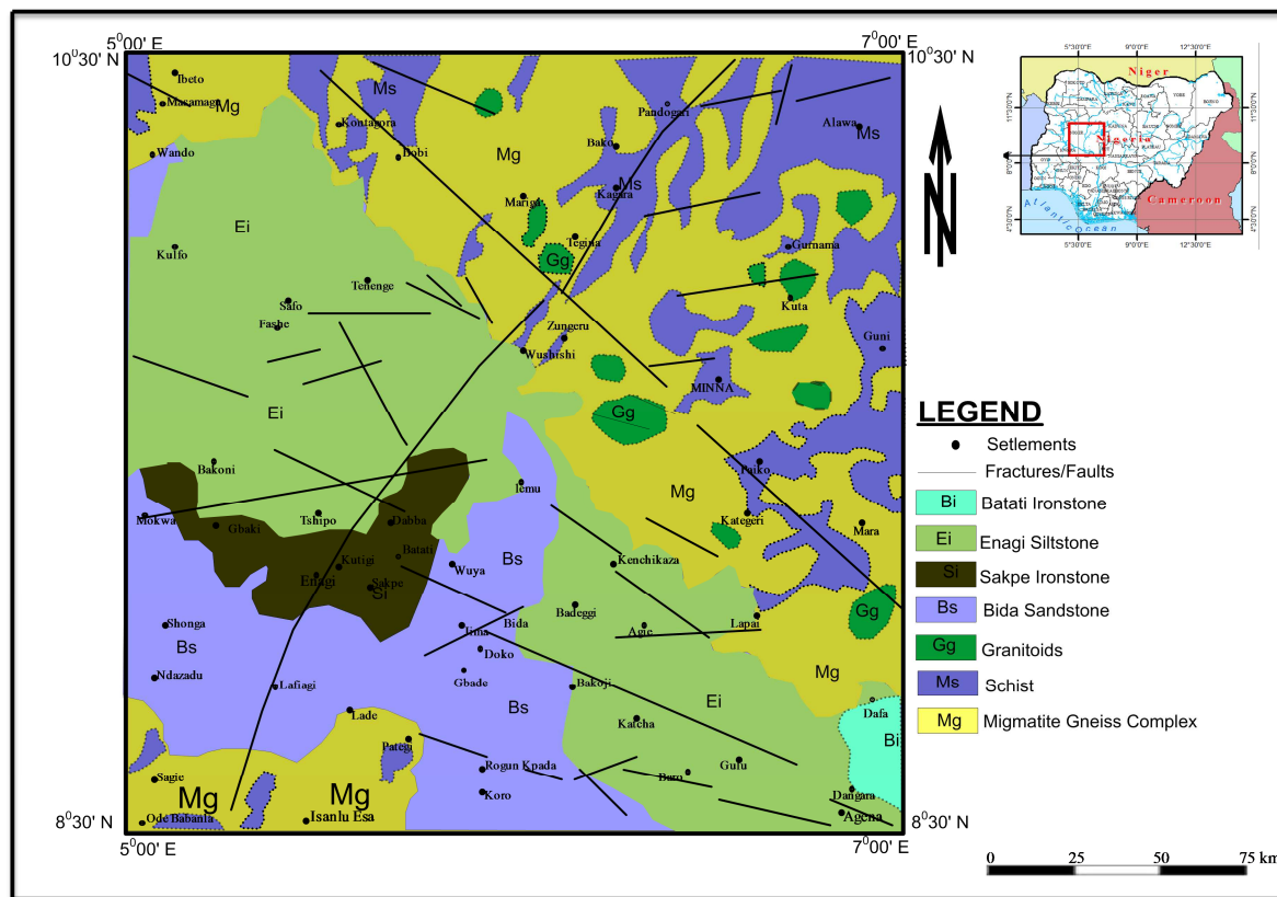
Fig. 10: Litho-magnetic and Structural Map of Northern Bida Basin and Environs
