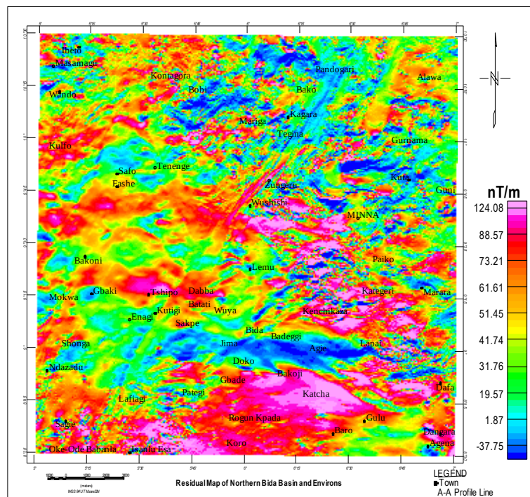
Fig. 3: Residual Map of Northern Bida Basin and Environs
