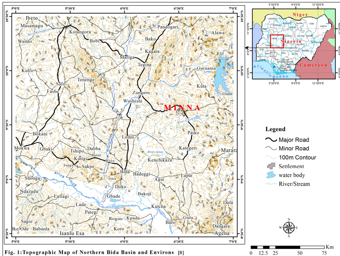
Fig. 1: Topographic Map of Northern Bida Basin and Environs [8]
