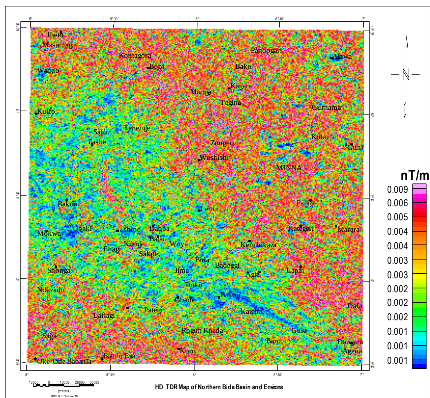
Fig. 7: Horizontal Derivative of TDR Map draped on the Study Area
