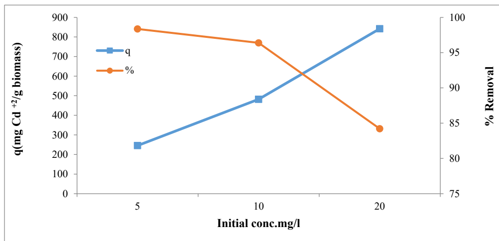
Fig (5): Effect of initial concentration on Cd (II) removal by S.baccularia at pH=6, T=30°C, 1g biomass
