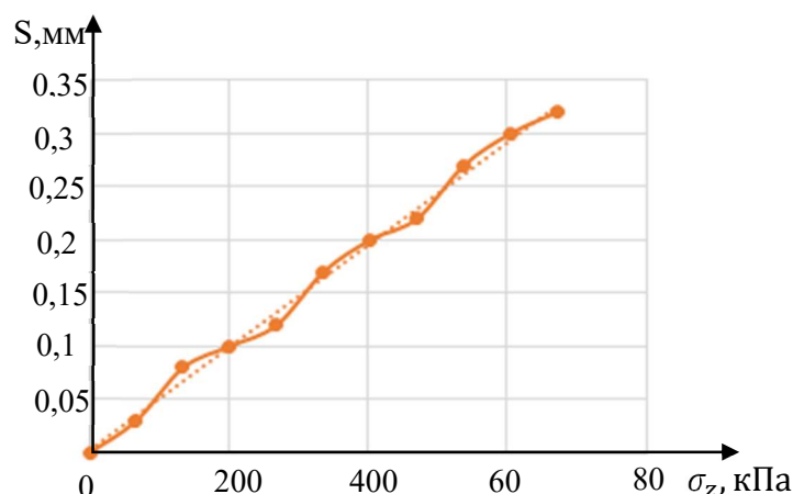
Fig.5. Calibration graph of the upset S versus axial pressure \sigma_z .
