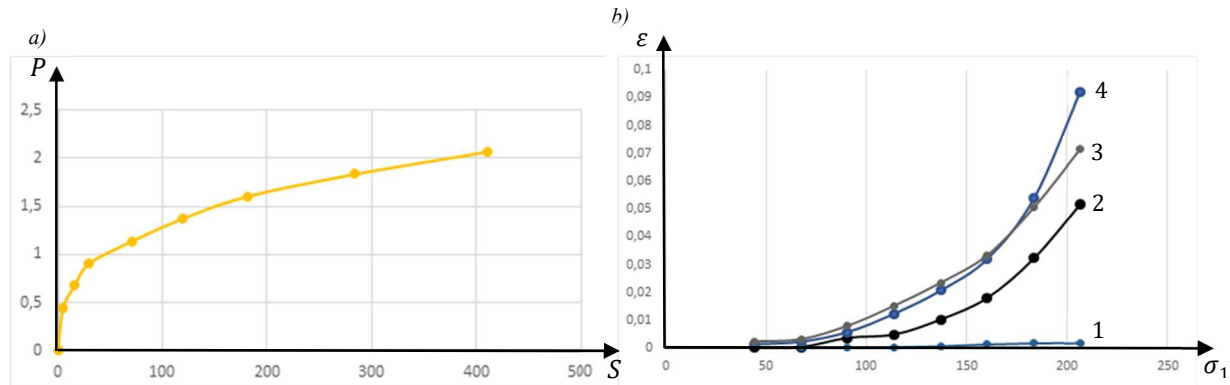
Fig.3.a) Vertical movement of the plate, mm; b) Lateral (horizontal) movements from the distance of the indicators from below; 1) indicator No. 1-10mm, 2) indicator No. 2-37mm, 3) indicator No. 3-102mm, 4) indicator No. 4-69mm.
