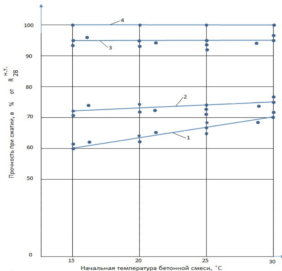
Figure: The nature of the increase in the strength of concrete on Portland cement, depending on the initial temperature of the concrete mixture, which underwent heat treatment according to the mode of 2 + 3 + 6 + 4 hours.
