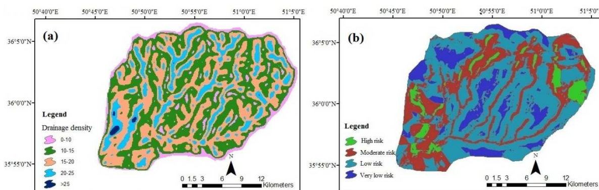
Fig. 14. (a) Drainage density, (b) the landslide hazard zonation map
