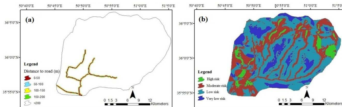
Fig. 16. a) Distance to road map, b) The landslide hazard zonation map.
