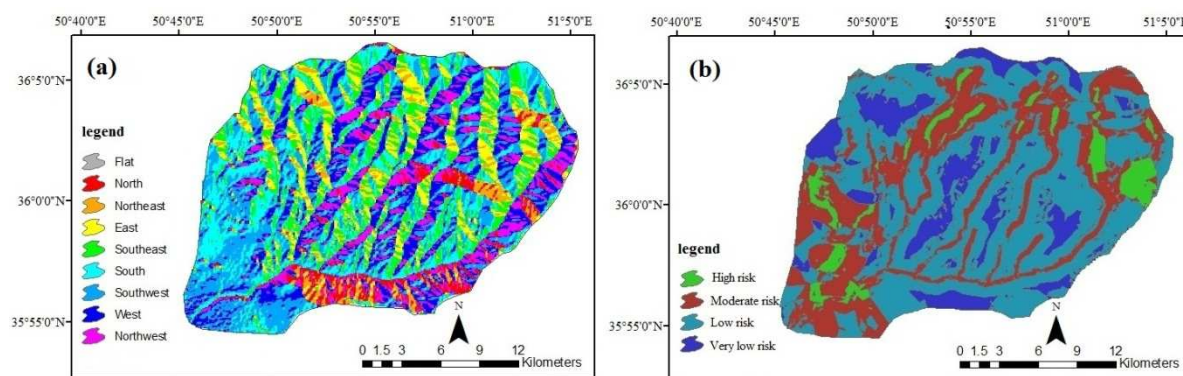
Fig. 18. a) Slope aspect map, b) The landslide hazard zonation map.
