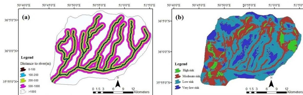
Fig. 8. a) Distance to rivers map b) The landslide hazard zonation map
