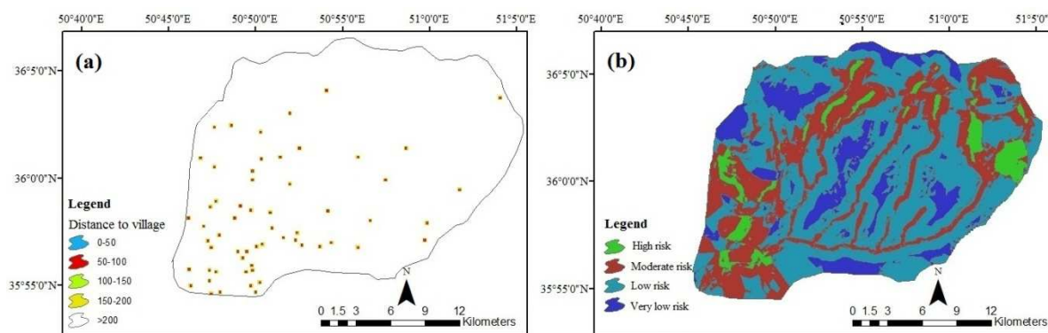
Fig. 12. a) Distance to villages, b) The landslide hazard zonation map.
