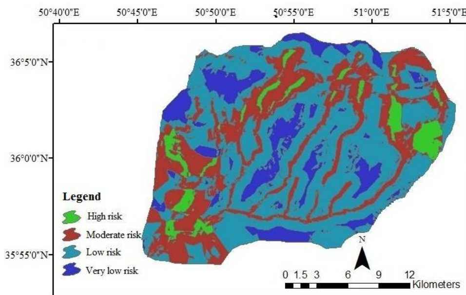
Fig. 6. The landslide hazard zonation map produced by the AHP.
