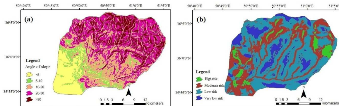
Fig. 15. a) Slope map, b) The landslide hazard zonation map.
