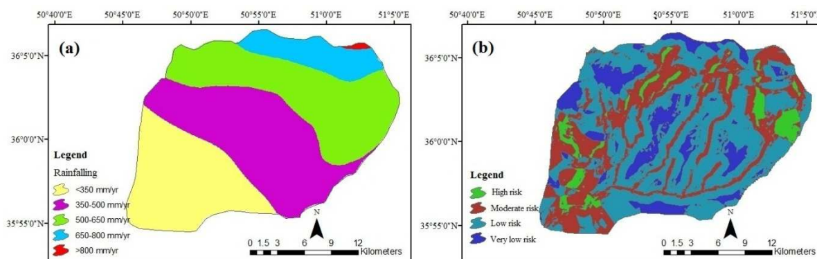
Fig. 11. a) isohyets map, b) The landslide hazard zonation map.
