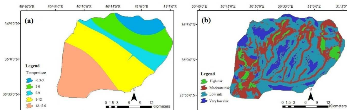
Fig. 19. a) isotherm map, b) The landslide hazard zonation map.
