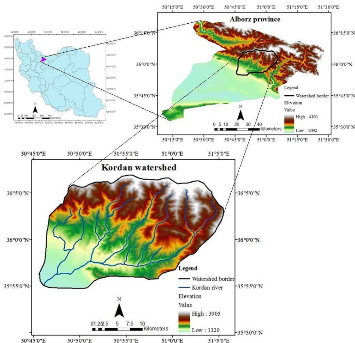
Fig.1. The location map of the study area in Iran.
