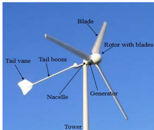
Figure 1. Main Components of Small Horizontal Axis Wind Turbine
