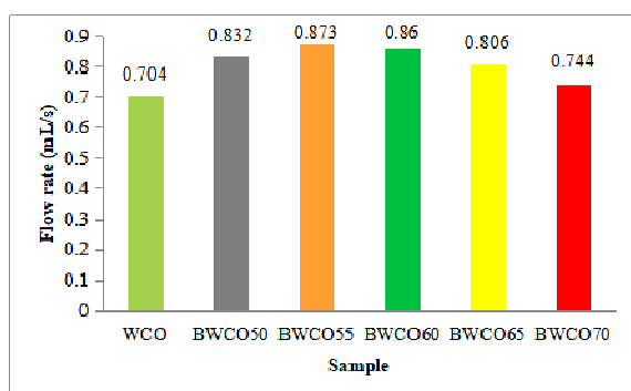
Fig. 3 Flow rates of biodiesel products and waste cooking oil
