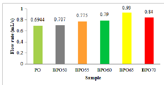
Fig.2 Flow rates of biodiesel products and palm oil (bimoli)
