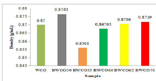
Fig. 5 Densities of biodiesel products and waste cooking oil
