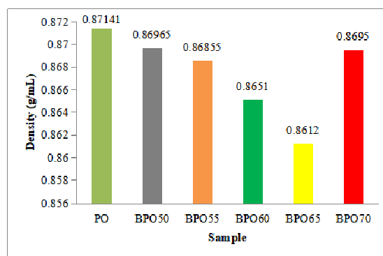
Fig. 4 Densities of biodiesel products and palm oil (bimoli)
