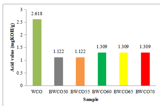
Fig. 7 Acid values of biodiesel products and waste cooking oil
